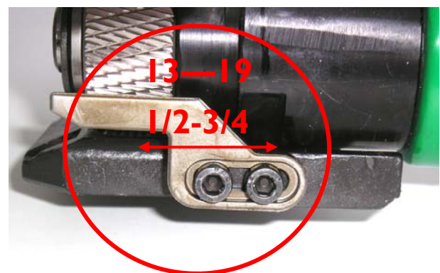
REAR GUIDE STRAP ADJUSTMENT- DETAIL
